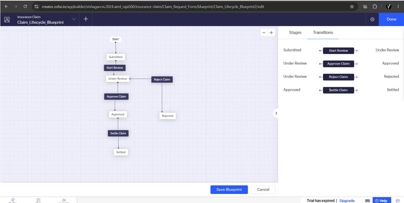
Figure 4 - Blueprint: Claim_Lifecycle_Blueprint showing stages and transitions.
