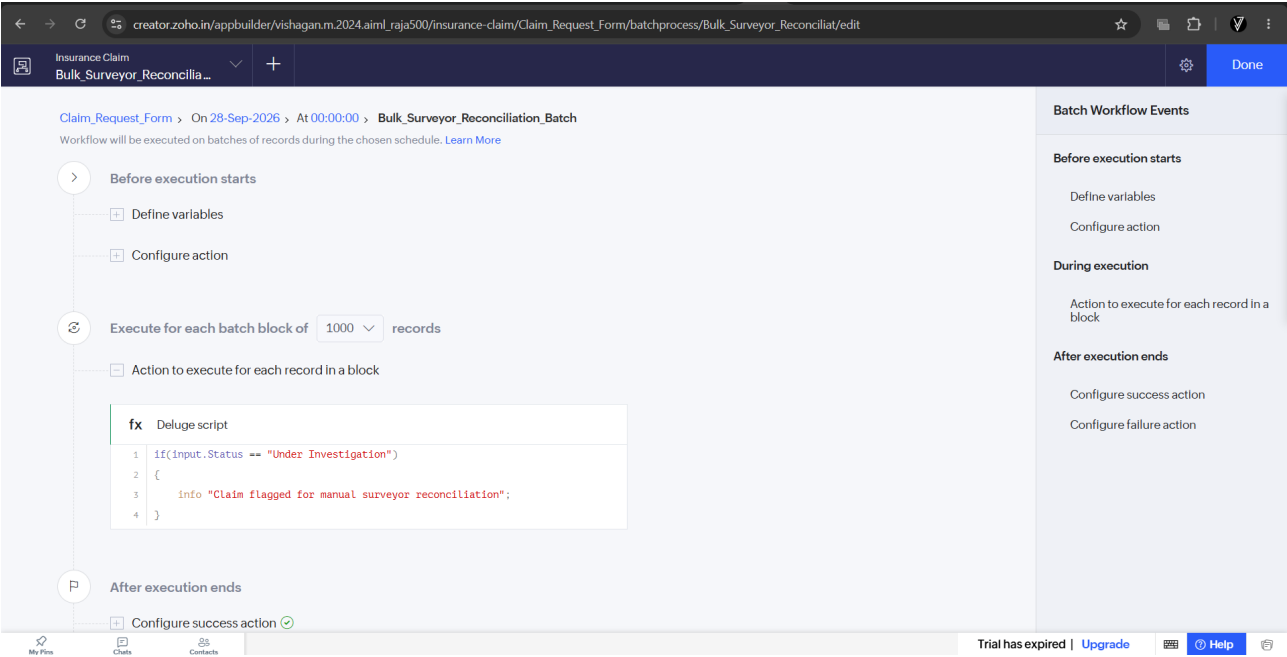
Figure 5 - Batch workflow: Bulk_Surveyor_Reconciliation_Batch with batch execution and Deluge action.
