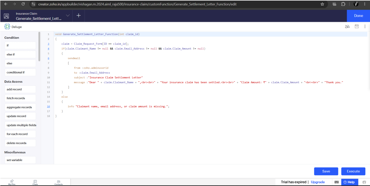
Figure 6 - Function: Generate_Settlement_Letter_Function with Deluge implementation.
